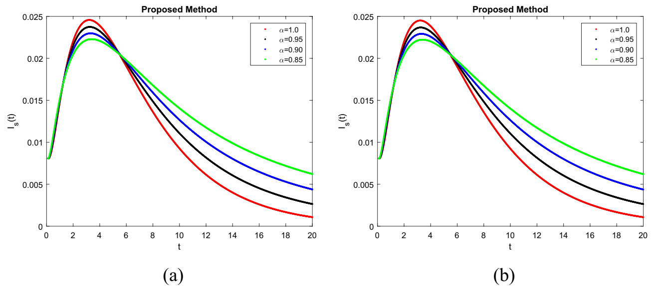
Figure 4. Simulation of I_s(t) . (a) p = 0.001 , (b) p = 0.0004 under the Caputo model.
