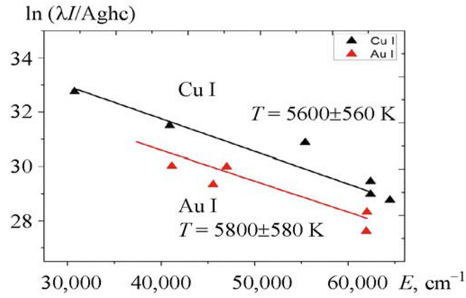
Fig. 3. Combined Boltzmann plots using lines of neutral gold (Au I) and copper (Cu I).
