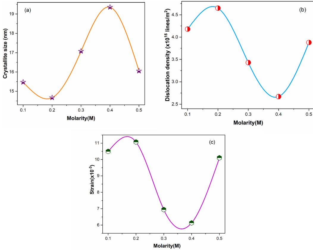
Fig. 3. Variation in (a) Crystallite size (b) dislocation density and (c) strain of magnesium iron oxide nanoparticles.
