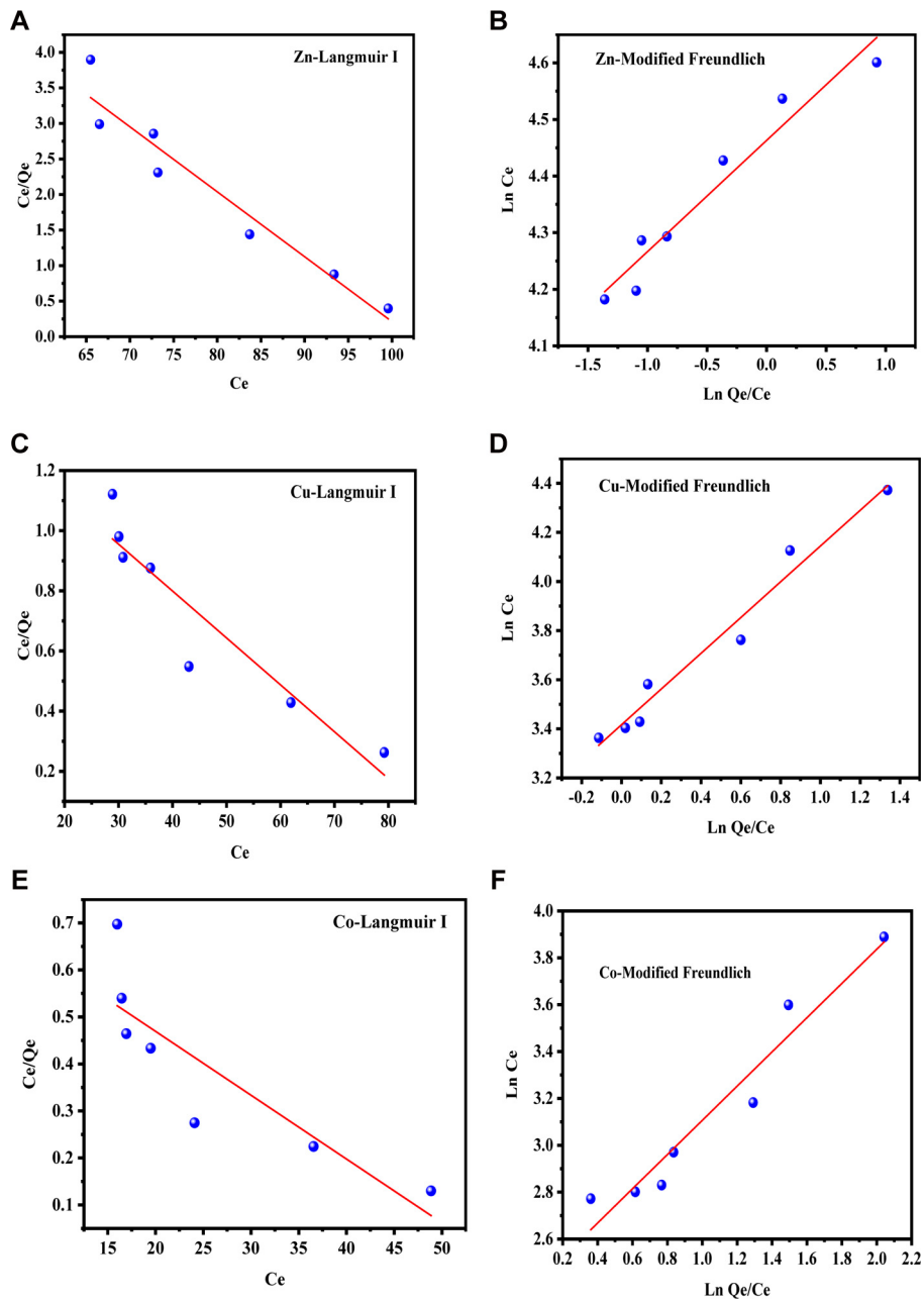
FIGURE 7 (A–F) Langmuir and Freundlich isotherm sorption models of Zn(II), Cu(II), and Co(II) on SBL from soil samples.
