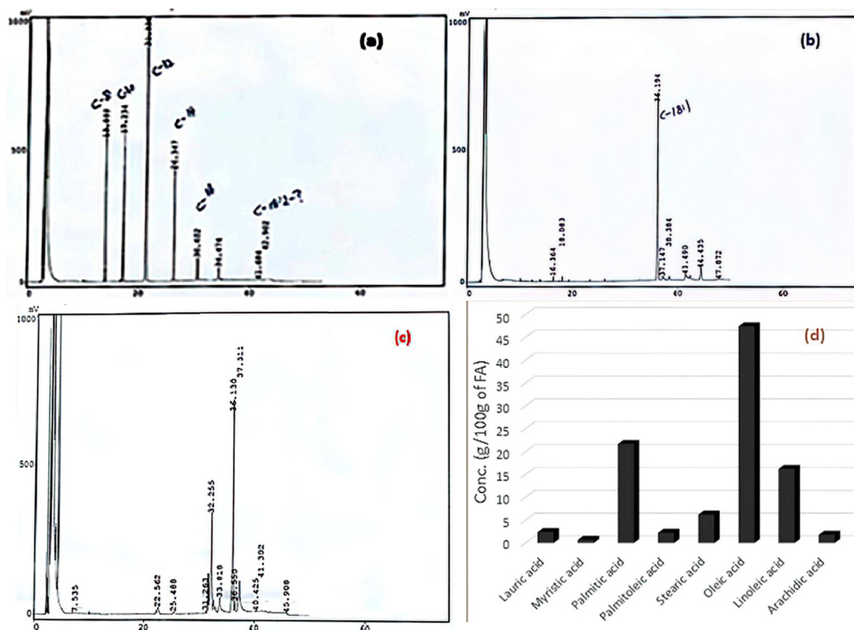
Fig. 1 Typical GC chromatograms: (a) saturated fatty acid standards, (b) unsaturated fatty acid standards, (c) wild olive oil FAMES, (d) quantitation of fatty acids.
