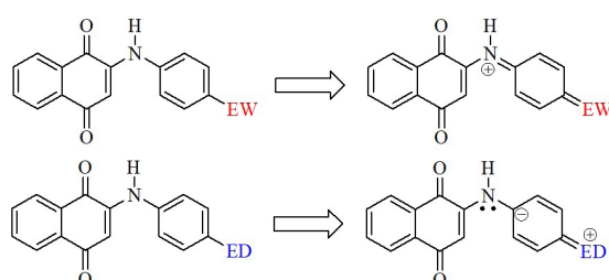
Scheme 2. Electronic effects of addition of e-withdrawing and donating groups on PAN compound (adopted [20] and redrawn).
