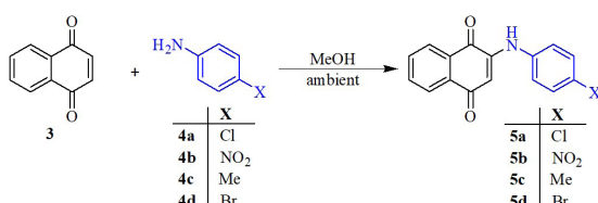
Scheme 1. Synthesis of 2-phenylamino-1,4-naphthoquinones derivatives.
