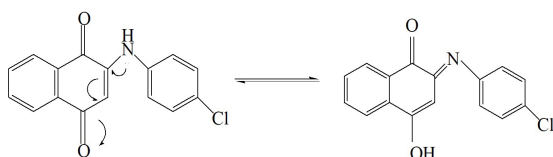
Figure 6. Proposed mechanism of action for chloro derivative of PAN.
