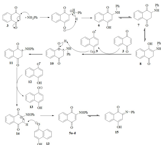
Scheme 4. Proposed mechanism of formation of 2-phenylamino-1,4-naphthoquinones.
