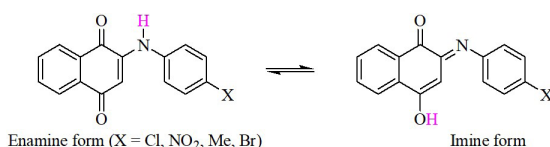
Scheme 3. Tautomeric form of 2-phenylamino-1,4-naphthoquinones (PAN) derivatives.
