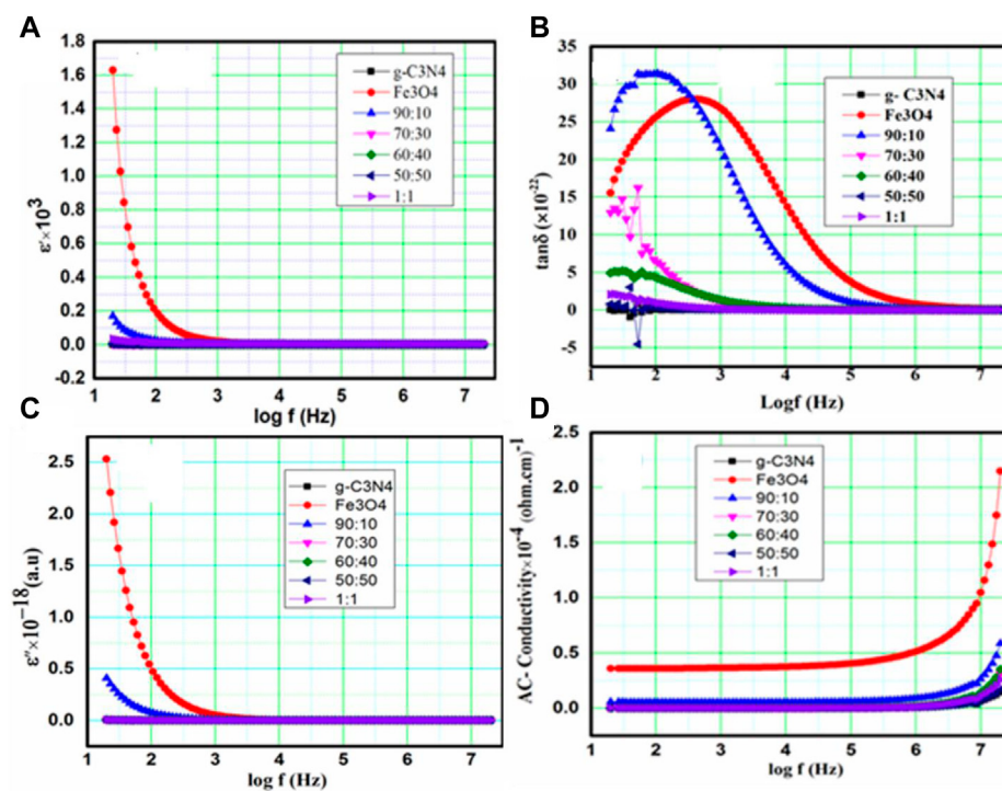
FIGURE 4 (A–D): Behaviors of the (A) dielectric constant ( \epsilon' ), (B) dielectric loss angle ( \tan\delta ), (C) dielectric loss factor ( \epsilon'' ), and (D) AC conductivity ( \sigma_{ac} ) for the applied material frequencies.
