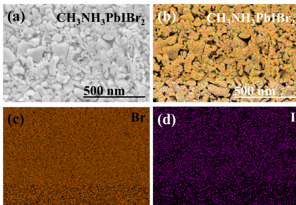
Figure 3. (a) Surface SEM analysis of multilayered top layer of \text{CH}_3\text{NH}_3\text{PbIBr}_2 thinfilm, (b) colored FESEM elemental analysis multilayered \text{CH}_3\text{NH}_3\text{PbIBr}_2 thinfilm, Dispersion of Br (c) and I (d).
