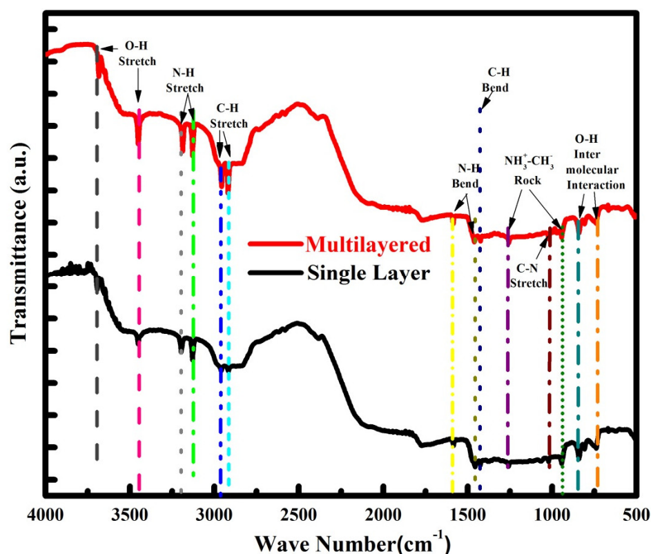
Figure 7. FTIR spectra for single-layer and multilayer \text{CH}_3\text{NH}_3\text{PbIBr}_2 thinfilms.
