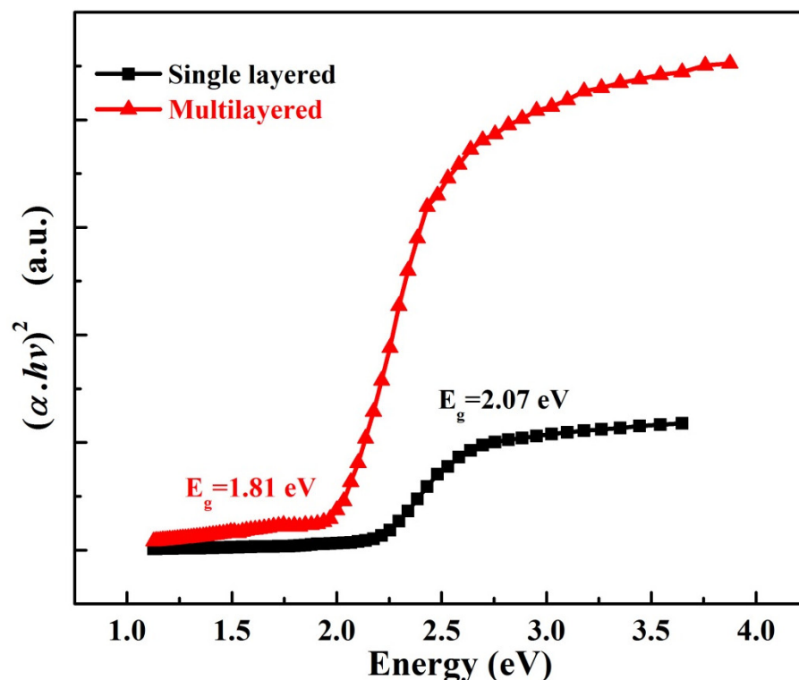
Figure 6. Tauc plot for single-layer and multilayered \text{CH}_3\text{NH}_3\text{PbIBr}_2 thinfilms.
