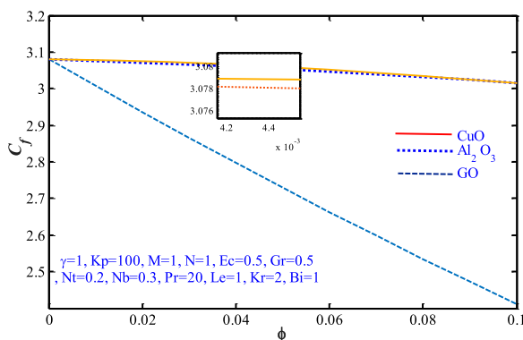
Figure 22. Skin friction variations against \phi for distinct nanoparticles.
