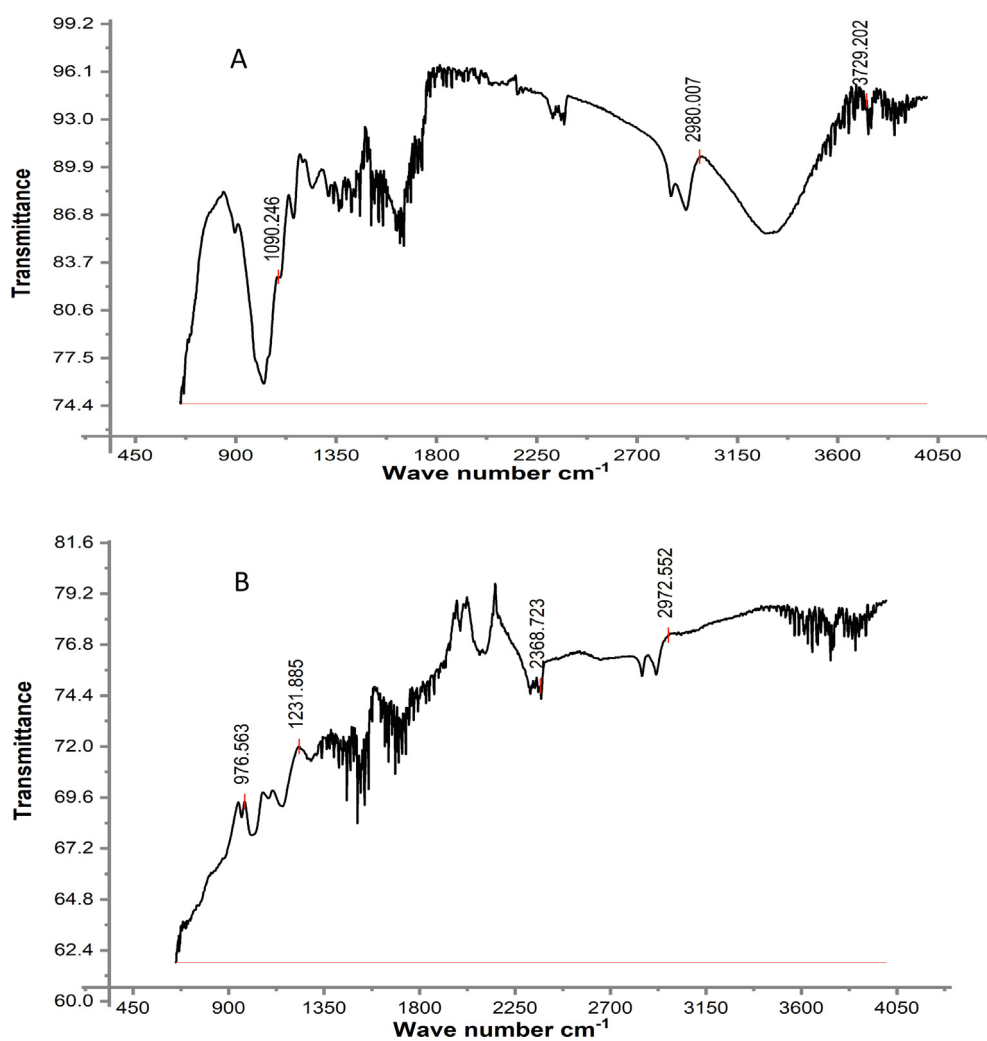
Fig. 7 FTIR analysis of RH adsorbent, (A) before adsorption (B) after adsorption.
