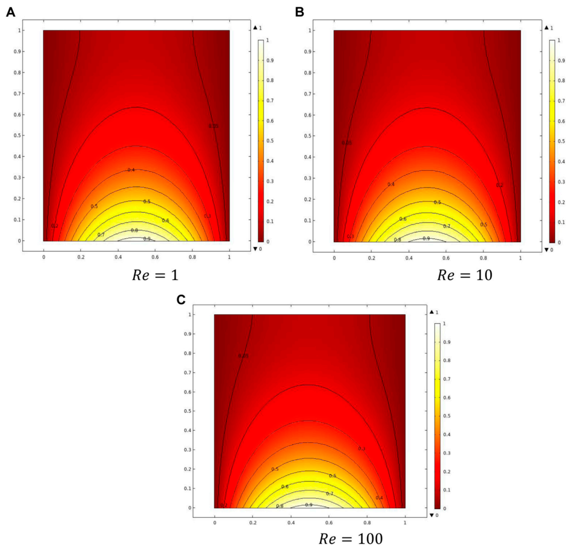
FIGURE 14 Influence of Re on the temperature profile for the non-uniform heating case. (A) Re = 1 , (B) Re = 10 , (C) Re = 100 .
