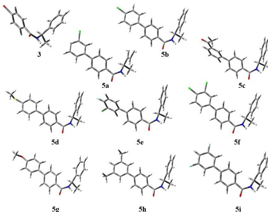
Figure 2. Optimized geometries of (3,5a–i) calculated at the B3LYP/6-311G (d,p)/SMD 1,4-dioxane level of theory.
