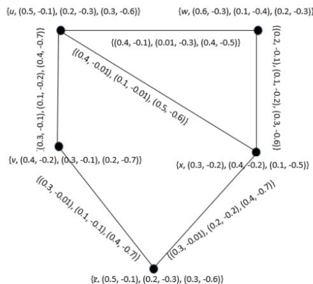
Figure 2: Bipolar Picture Fuzzy Graph
