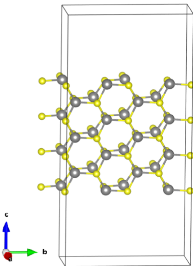
Figure 7. Schematic of the (11-20) surface slab model with seven CdS layers; the gray and yellow balls denote the Cd and S atoms, respectively.
