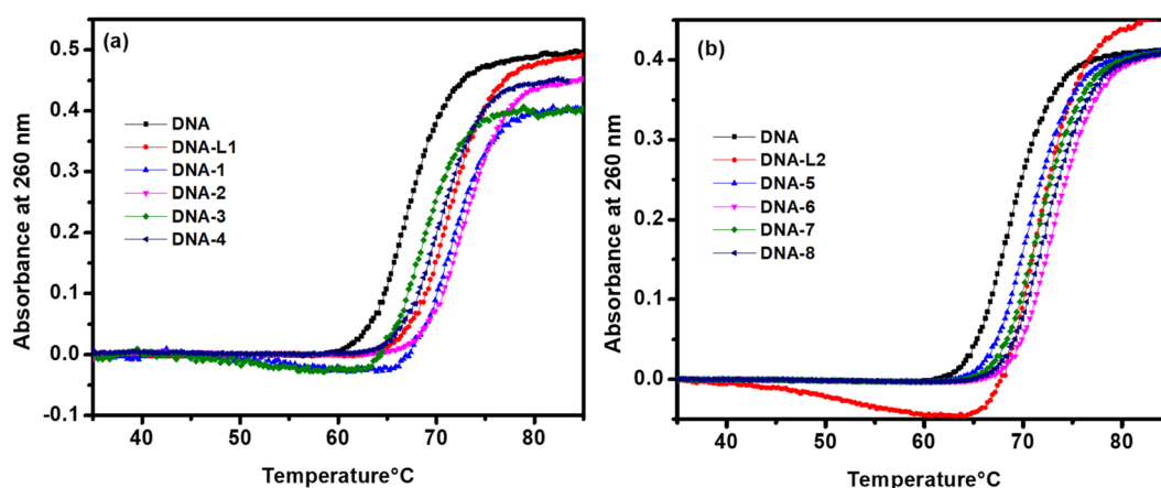
Fig. 8 Melting curves for 100 μM of ST-DNA upon the addition of ligand L_1 and complexes 1–4 (a), ligand L_2 and complexes 5–8 (b).
