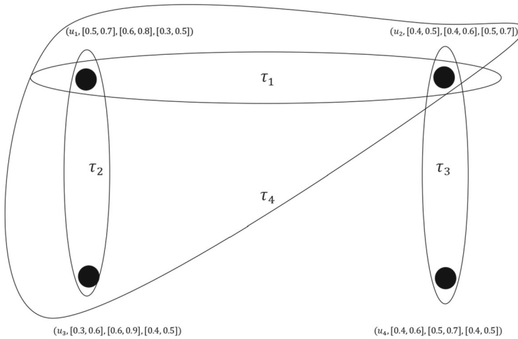
Fig. 3 Interval-valued picture fuzzy hypergraph
