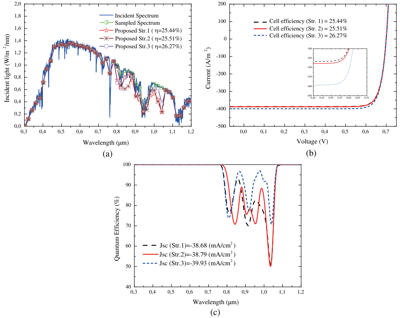
Figure 5. (a) absorption spectrum, (b) solar cell J-V curve, (c) quantum Efficiency Vs wavelength, for the three structures.
