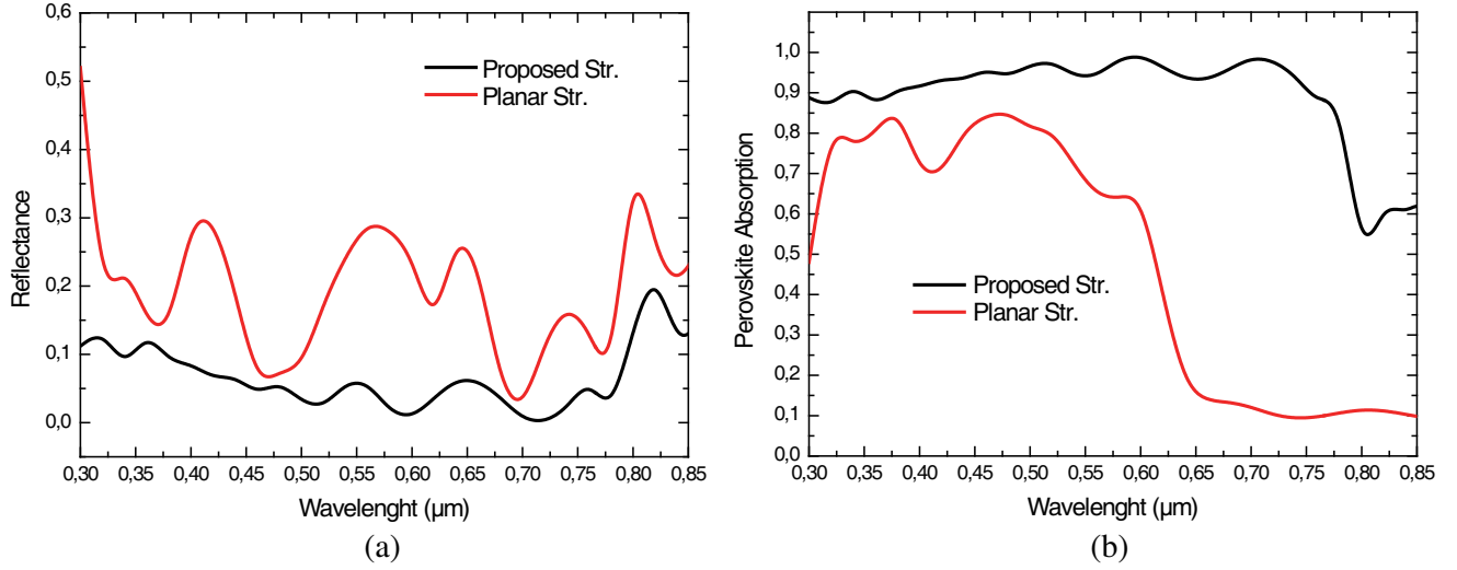
Figure 2. (a) Normalized reflectance and (b) absorption spectra, for planar and proposed structures.
