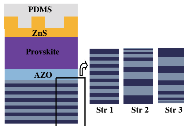
Figure 4. Perovskite-based solar cell with PhC-1D ( \text{Ge/SiO}_2 ) with different configurations of layer PhC-1D layers, ( Str 1 ) The thickness of layer PhC-1D is equal, ( Str 2 ) The thickness of layer PhC-1D is from smallest to largest, ( Str 3 ) The thickness of layer PhC-1D is from largest to smallest.
