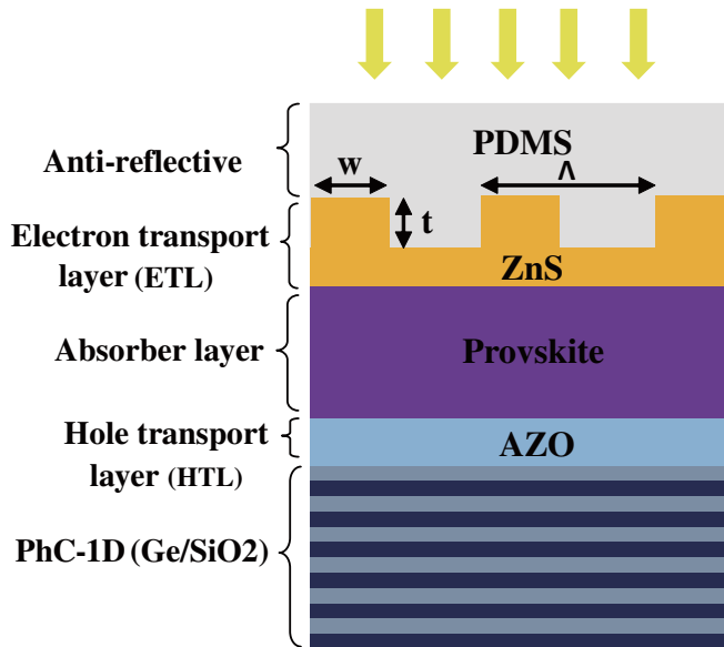
Figure 1. Proposed perovskite-based solar cell structure.
