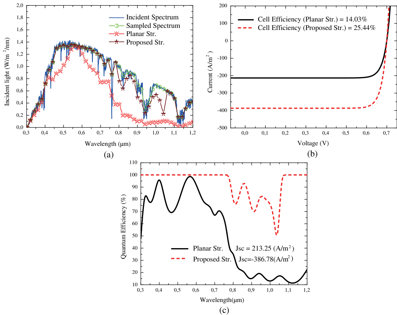
Figure 3. (a) Absorption spectrum, (b) solar cell J-V curve and (c) quantum efficiency Vs wavelength.
