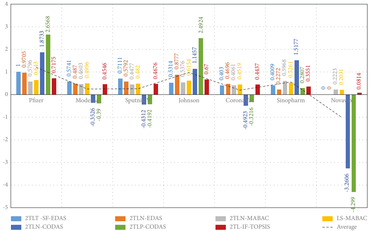
FIGURE 4: Comparative outcomes with the 2TL T -SFWMSM operator.
