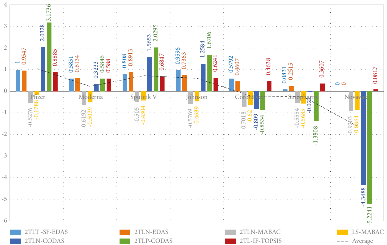
FIGURE 5: Comparative outcomes with the 2TL T -SFWDMSM operator.
