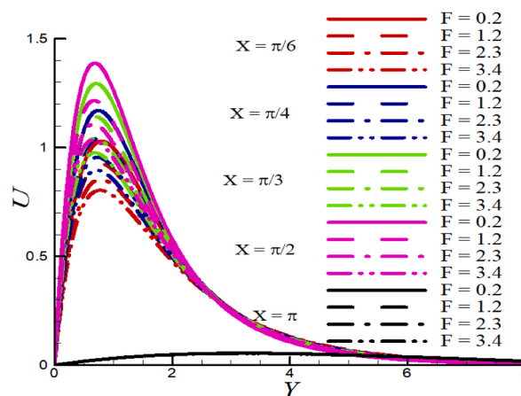
Fig. 2. Impact of F on U when Pr = 7.0 , N_r = 1.0 , H = 1.0 , and D = 0.1 .
