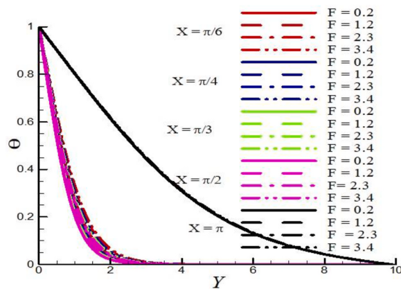
Fig. 3. Impact of F on \theta when R_g = 10.0 , Pr = 7.0 , N_r = 1.0 , H = 1.0 , and D = 0.1 .
