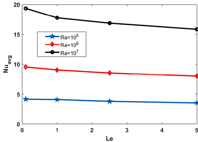
Fig. 6. Variation in average Nusselt number for different values of Ra and i Lewis number ( Le ) for Pr = 6.8 , Ha = 25 , \beta = 1 , N = 1 and \gamma = 30^\circ .
