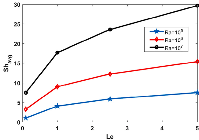
Fig. 7. Variation of average Sherwood number for different values of Ra and Lewis number ( Le ) for Pr = 6.8 , Ha = 25 , \beta = 1 , N = 1 and \gamma = 30^\circ .
