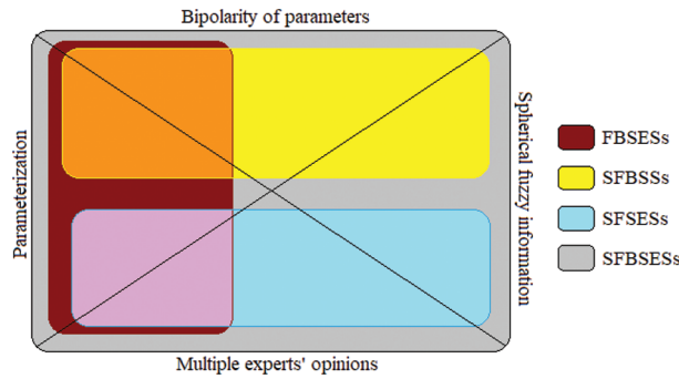
Figure 5: SFBSESs vs. FBSESs, SFSESs, and SFBSSs
