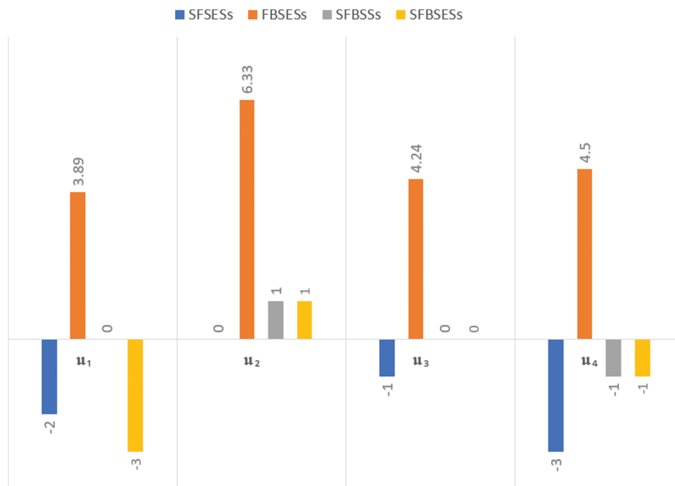
Figure 6: Scores comparison by SFSEs, FBSEs and SFBSEs
