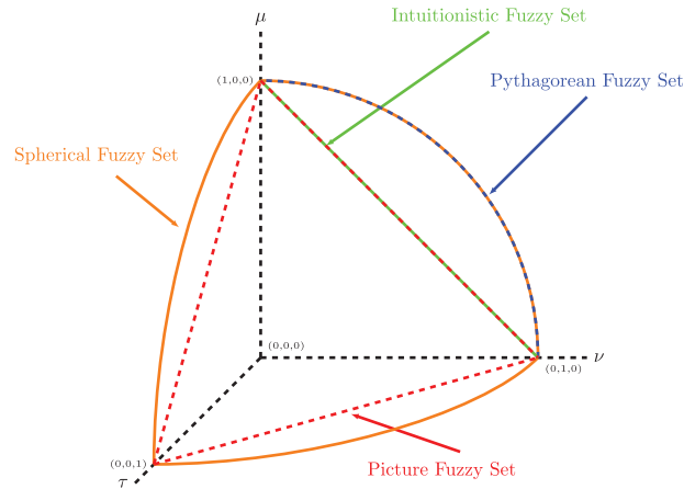
Figure 1: Pictorial representation of IFS, PyFS, PFS, and SFS
