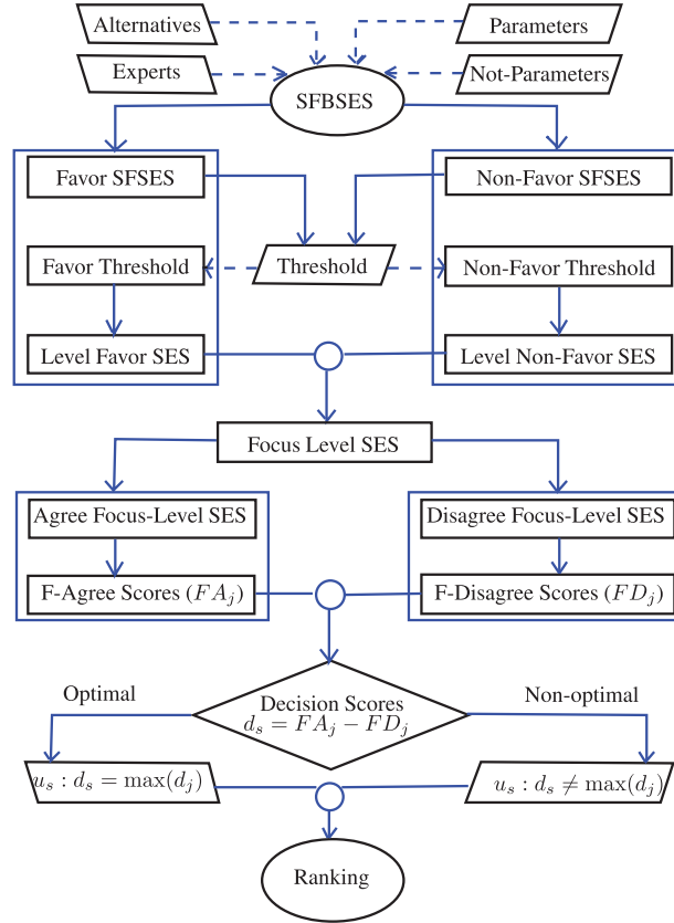
Figure 2: Multi-attribute group decision-making under SFBSEs
