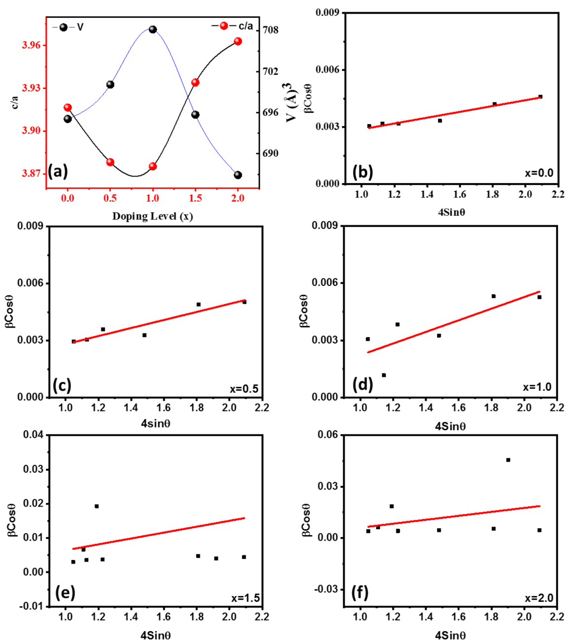
Fig. 2 a c/a ratio and volume (V) vs different doing levels of \text{Ba}_{0.8}\text{In}_{0.2}\text{Fe}_{12-x}\text{Ni}_x\text{O}_{19} hexaferrites. b–f W–H plots for the \text{Ba}_{0.8}\text{In}_{0.2}\text{Fe}_{12-x}\text{Ni}_x\text{O}_{19} hexaferrites
