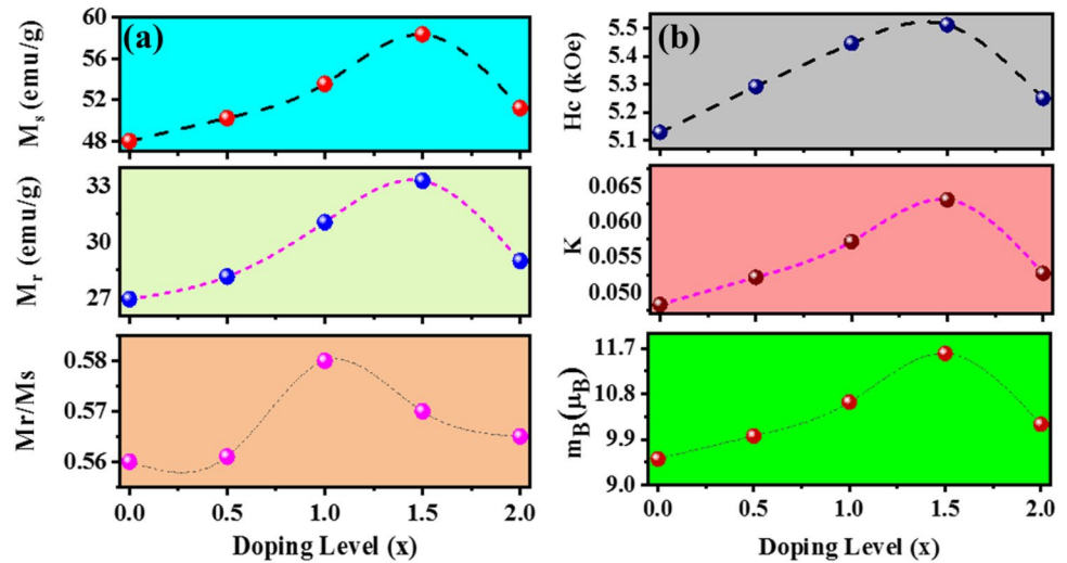
Fig. 6 a Variance in M_s , M_r , M_r/M_s vs doping level ( x ). b Variation in H_c , m_B , and K for different doping levels in \text{Ba}_{0.8}\text{In}_{0.2}\text{Fe}_{12-x}\text{Ni}_x\text{O}_{19} hexaferrites
