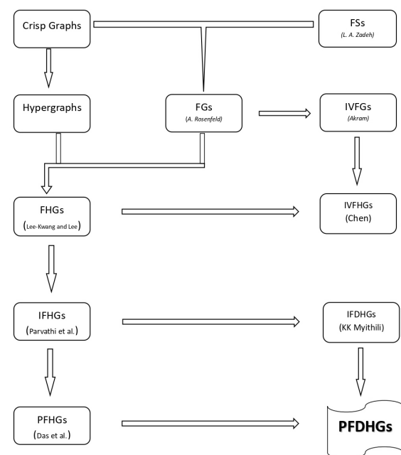
FIGURE 1. Generalizations of Fuzzy hypergraphs.
