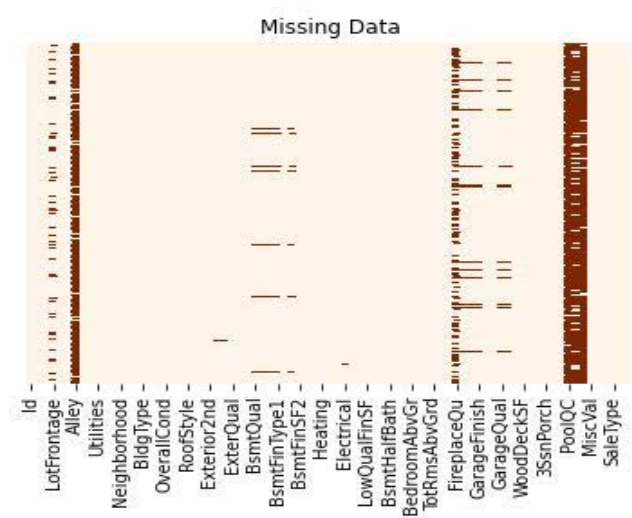
FIGURE 4. Seaborn heatmap.
