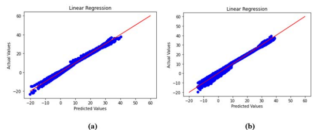
FIGURE 21. Scatter plot of weather in Szegeed 2006-2016 dataset (a) after auto preprocessing of dataset, and (b) after manually preprocessing of dataset.
