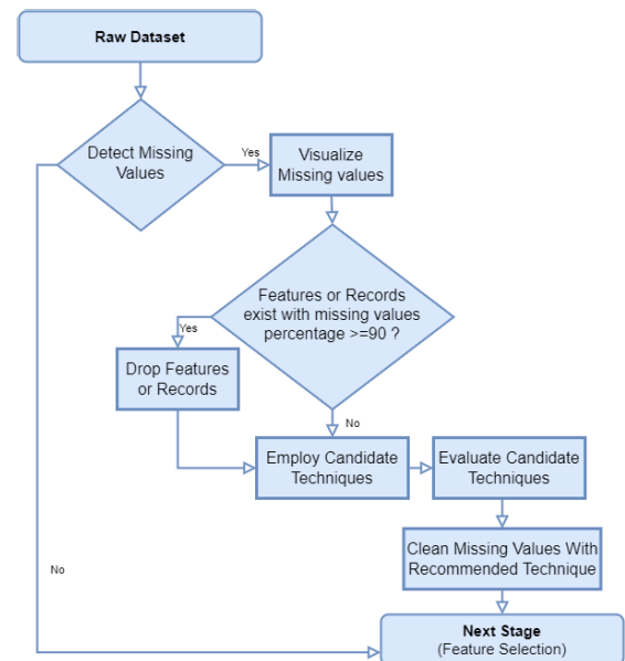
FIGURE 2. Workflow of automatic missing values handling.
