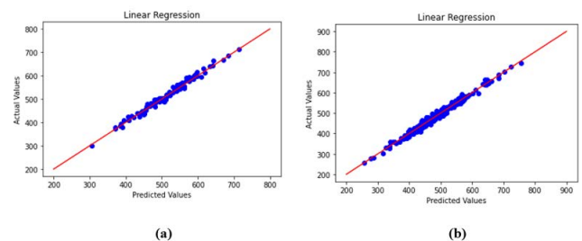
FIGURE 19. Scatter plot of ecommerce customers dataset (a) after auto preprocessing of dataset, and (b) after manually preprocessing of dataset.
