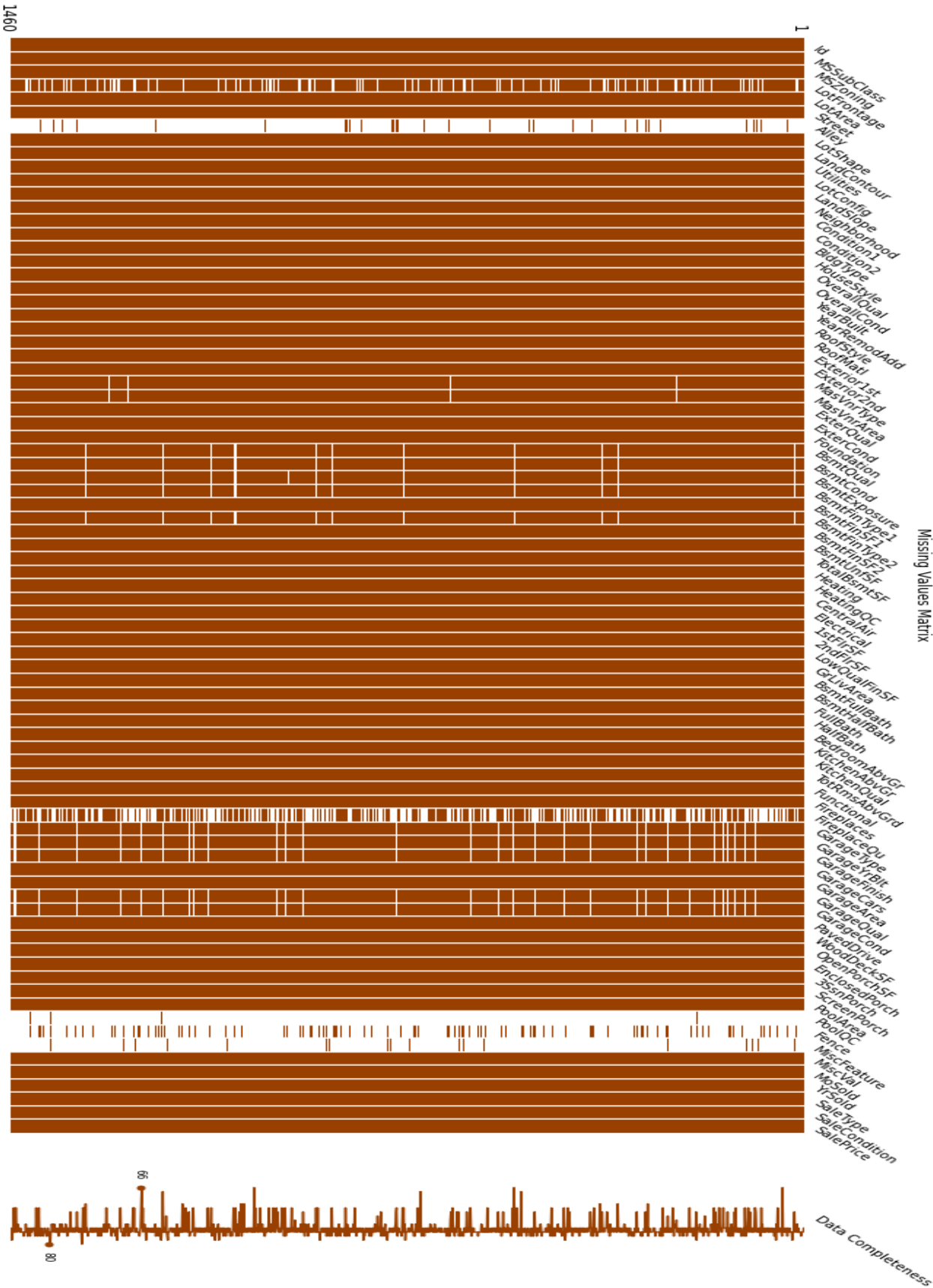
FIGURE 5. Missingno matrix.
