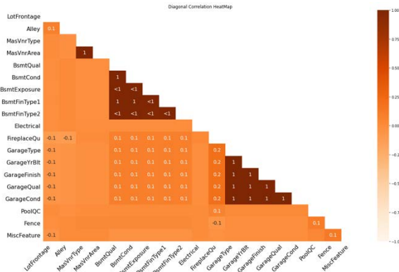
FIGURE 6. Missingno heatmap.
